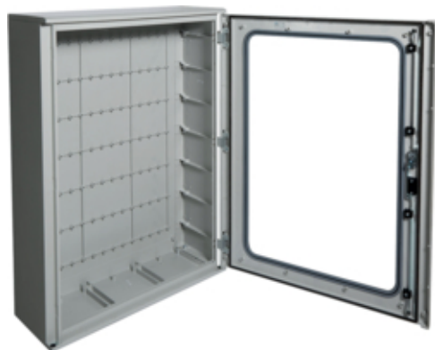
Armoire, orion plus, murale, single polyester, 1150x1100x300mm
